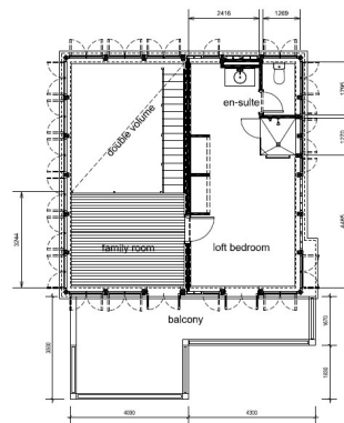
Loft floor plan:
